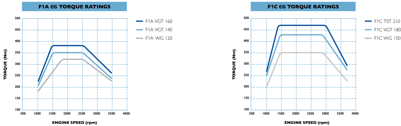
VGT: Variable Geometry Turbocharger; WG: WasteGate; TST: Twin Stage Turbocharger
